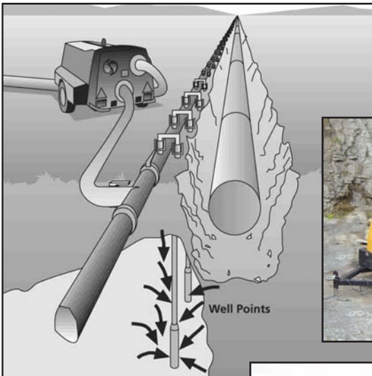
Sewer Bypass Well Point Dewatering Location Dewatering
