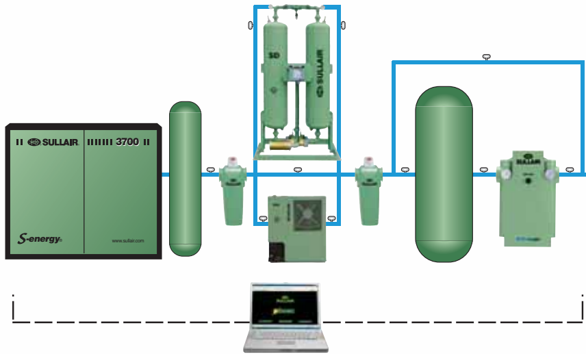
The Sullair System here includes: a Sullair compressor, "wet" receiver, Sullair pre-filter, your choice of a Sullair Desiccant or Refrigerated Air Dryer, Sullair after-filter, "dry" receiver, and Sullair Flow Controller. Monitoring and controlling the entire system is Sullair's PC-based eConnect TM .
