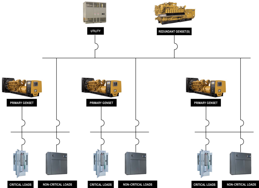
Figure 2: Example of Modular DC Configuration
